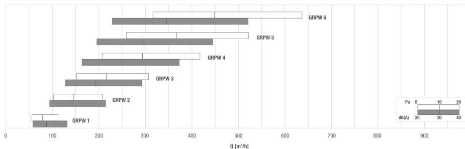
DIAGRAMMA SCELTA RAPIDA - QUICK SELECTION DIAGRAM
