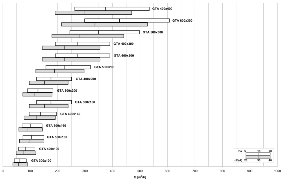
DIAGRAMMA SCELTA RAPIDA / QUICK SELECTION DIAGRAM
